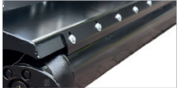
The scraper keeps the support roller clean and reduces dust development (optional).
