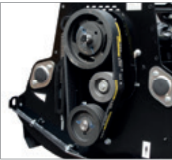
Trouble-free and low-maintenance operation due to the efficient design of the automatic belt tensioning system.
