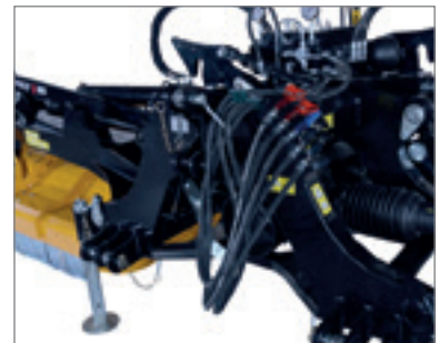
Tidy: The on-board hydraulics with the hydro-pneumatic MU-SOFA® weight transfer system.
