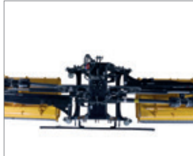
The clever offset design allows for a high-performance twin gear box and split power transmission to each side.
