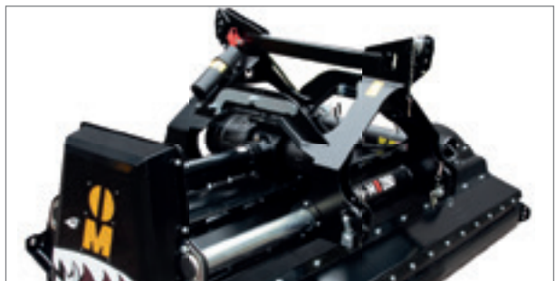
Sturdy front/rear attachment with hydraulic side shift (56 cm adjustment travel).
