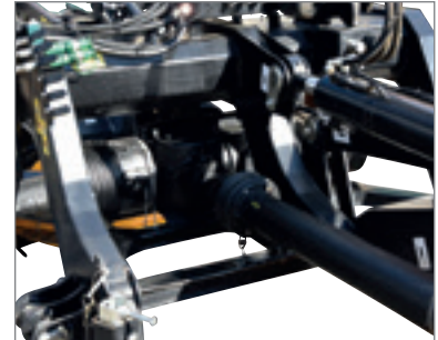
The gear box: Designed for driving powers of up to 400 HP.
